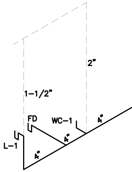
TYPICAL RR ISOMETRIC: N.T.S.
