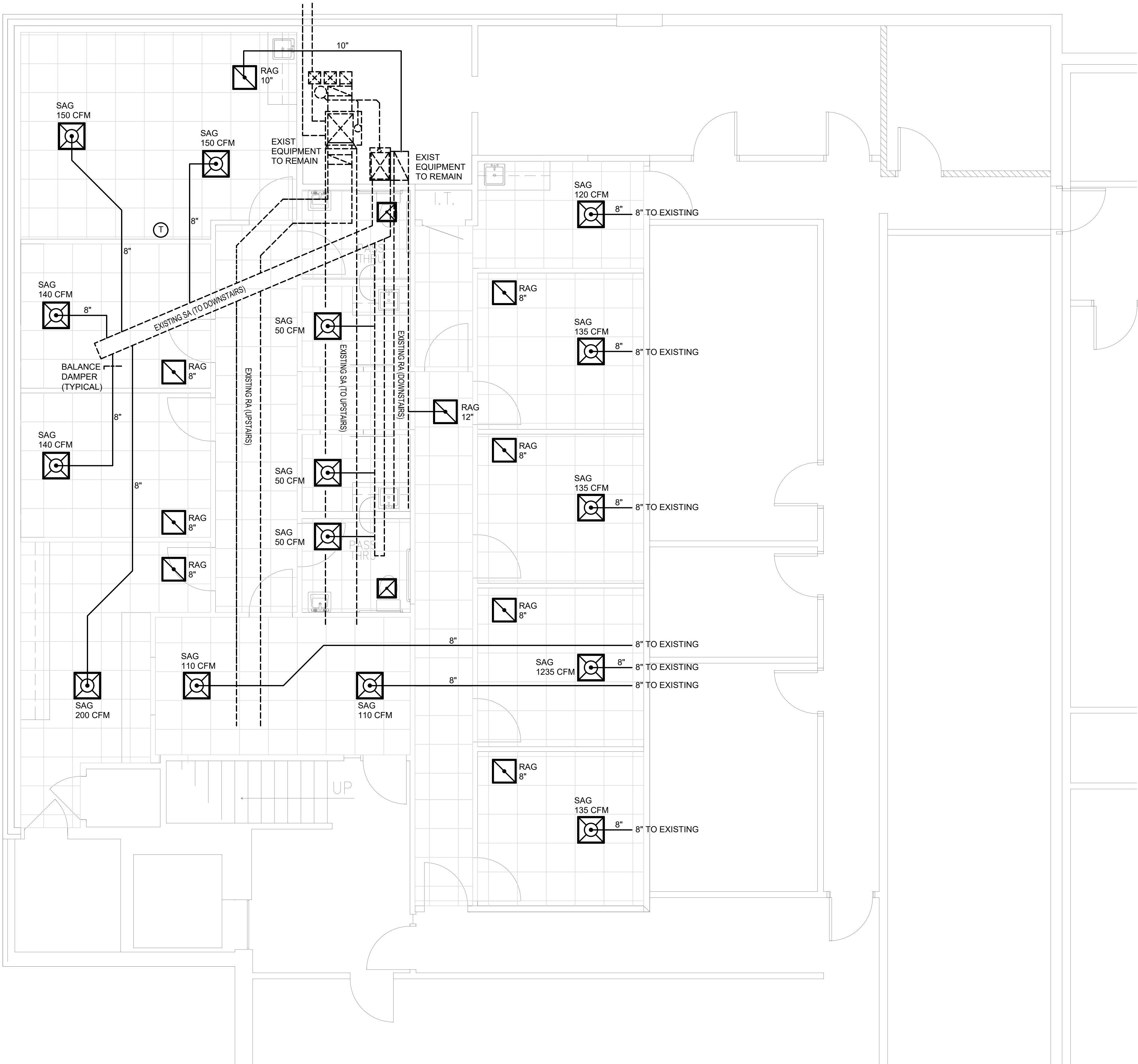
MECHANICAL HVAC PLAN: SCALE: 1/4" = 1'-0"
