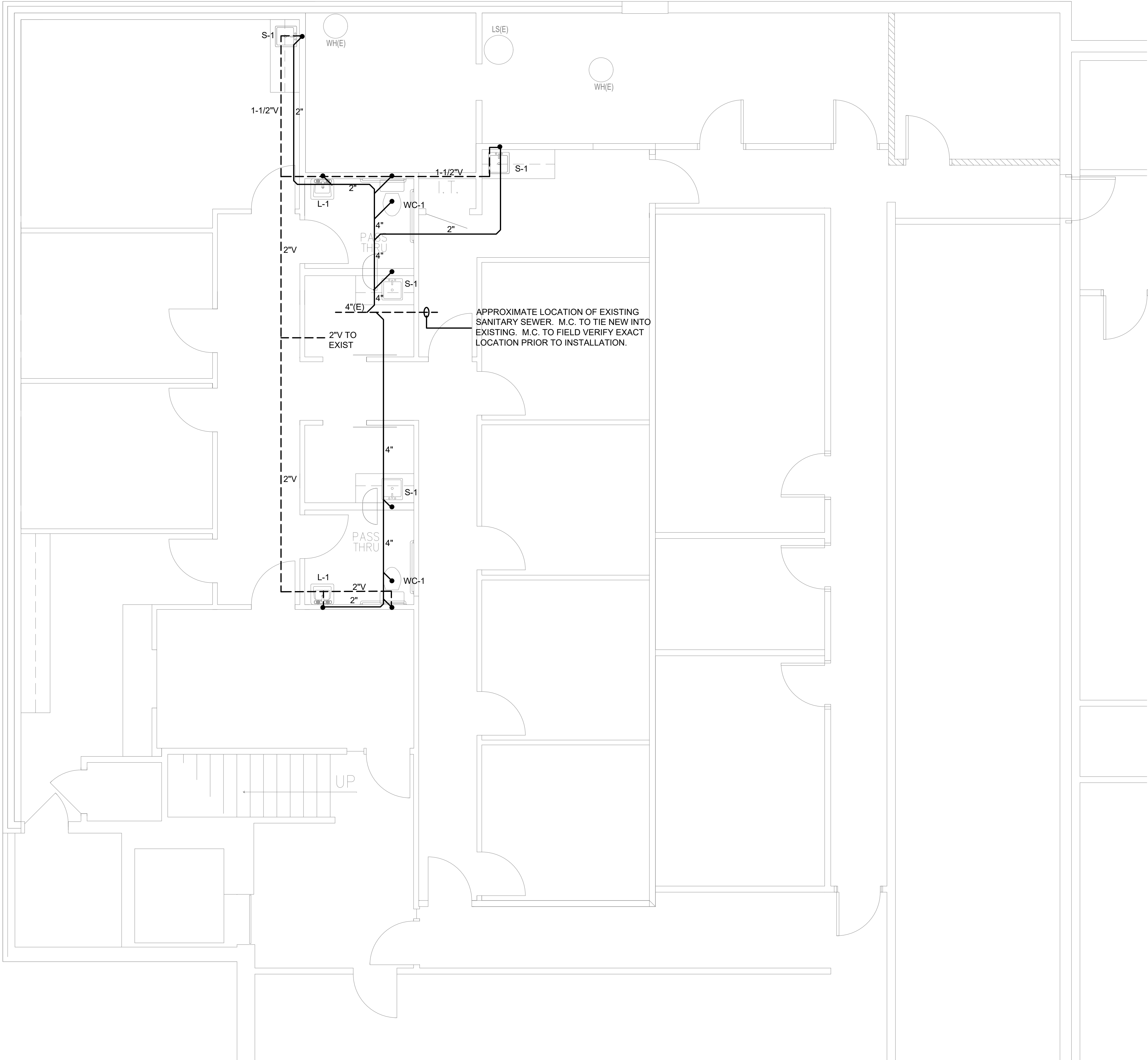
MECHANICAL PLUMBING PLAN: SCALE: 1/4" = 1'-0"
